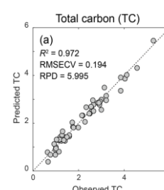
Better predictive accuracy of ISE-PLS in soil total C estimation
